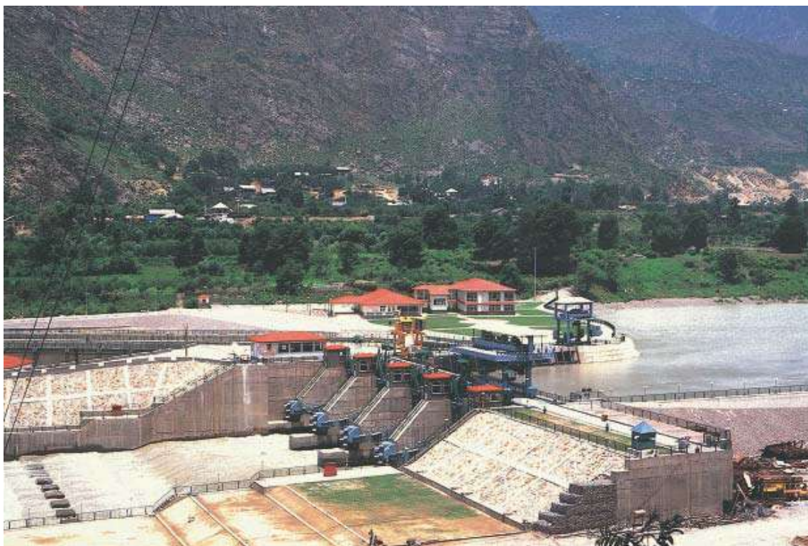
Baspa HEP - A view of the Diversion Barrage in Distt. Kinnaur, across Baspa river at Kuppa, H.P.
